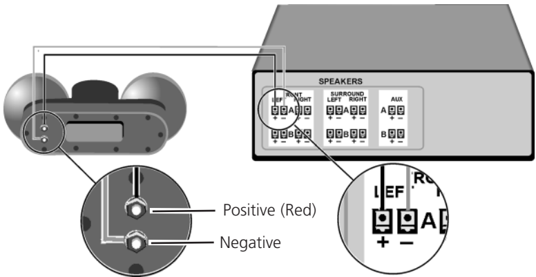
Figure 6. Loudspeaker Connections
