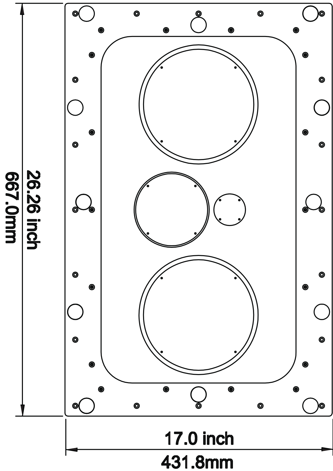
Front Baffle Dimensions
