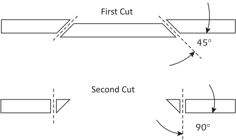
SIDE VIEW OF CEILING
