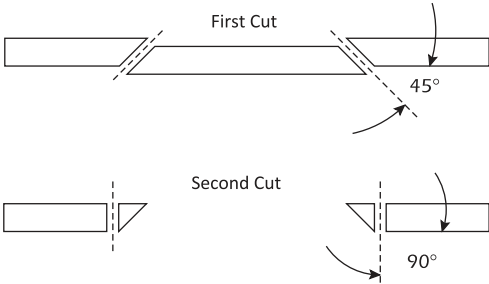
SIDE VIEW OF CEILING
