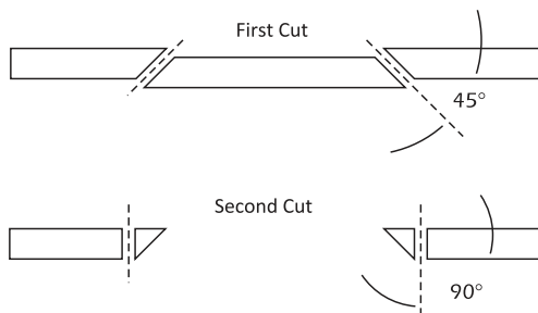
SIDE VIEW OF CEILING
